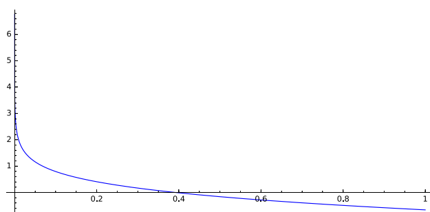
Figure A1. The plot of \hat{h}_{\text{appr}} = \sum_{i=0}^{19} \mathcal{L}_\eta f_\eta .
