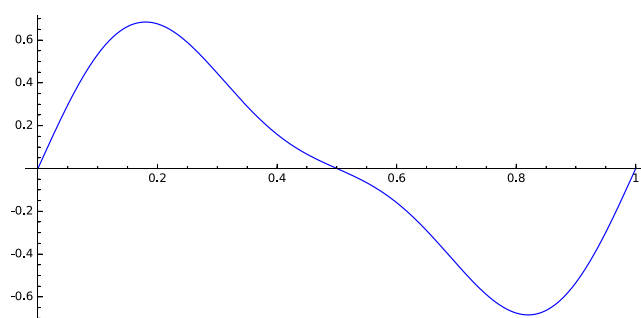
Figure 2. The plot of \hat{h}_{\text{appr}} = \sum_{i=0}^{56} \mathcal{L}_\eta f_\eta .
