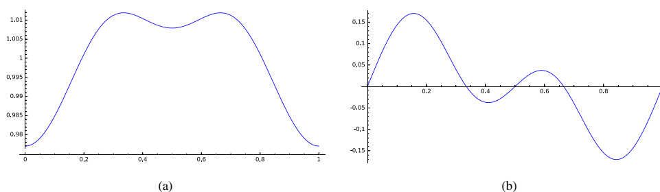
Figure 1. The computed approximations of the response in the stochastic case, and a plot of an approximation of the invariant density for the non-perturbed map. (a) A plot of the invariant density. (b) The computed linear response.
