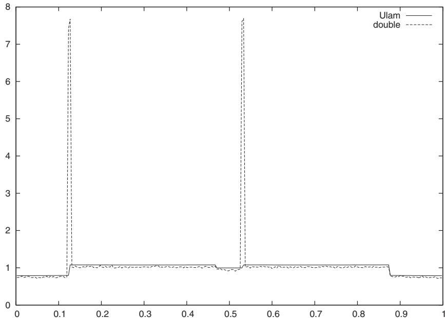
Fig. 5. 1,000,000 Iterates: Birkhoff averages and Ulam approximation
